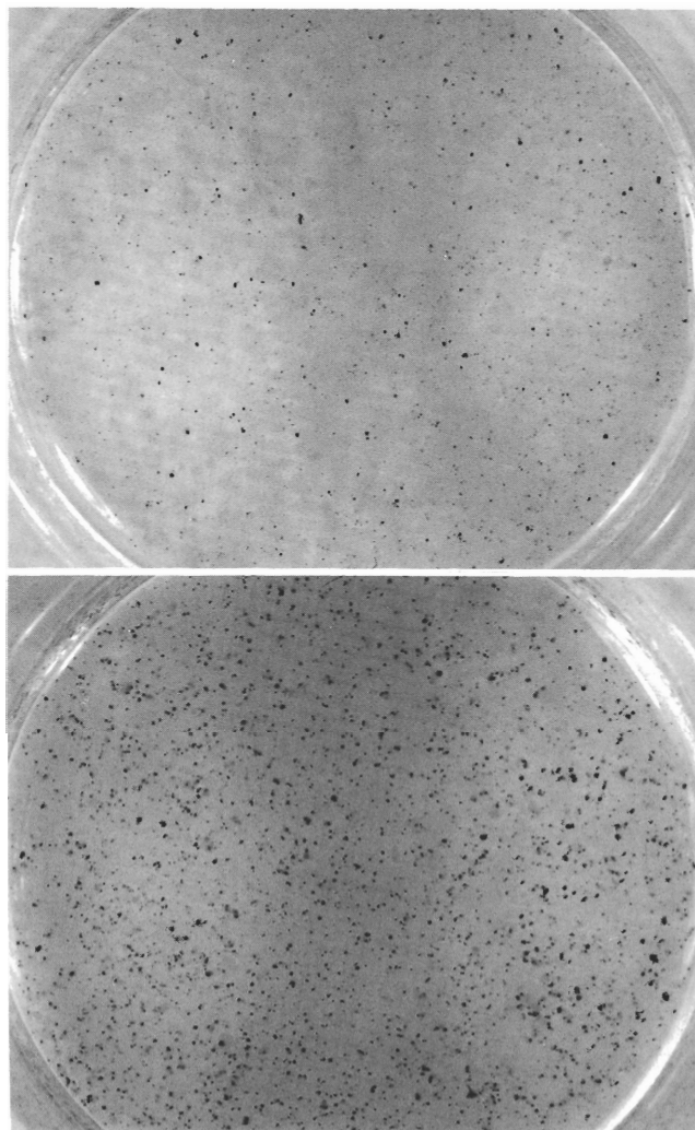
Figure 1. GUS expression in embryogenic maize cells 2 d after bombardment: a) without osmotic treatment b) with osmotic treatment (0.4 M osmoticum).
